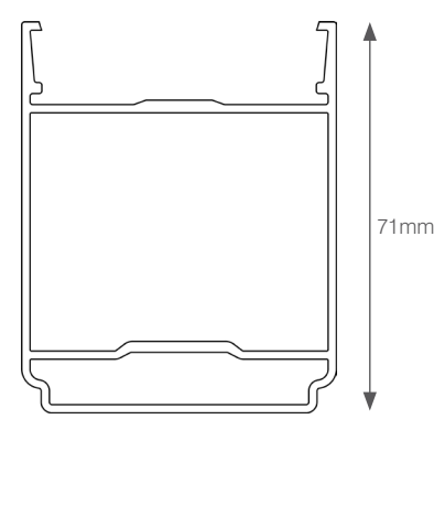
RAFTER BODY KLP-03
