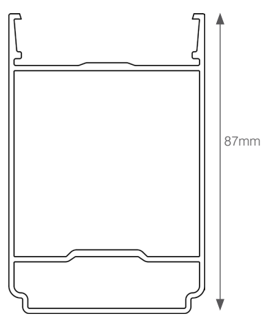
RIDGE BODY KLP-01
