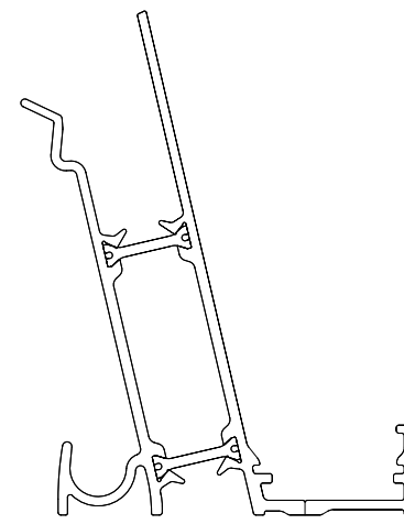
EAVES BEAM KLP-05
