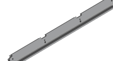
EAVES BEAM KLP-05
